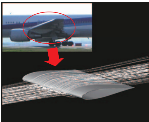
乱流中の翼周りの流れ (粒子軌跡) Flow (particle trajectories) around an aerofoil in a turbulent flow
