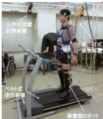
装着型ロボット装着時歩行計測実験 Measurement of the Gait Motion of A Human Wearing A Physical Assistant Robot
