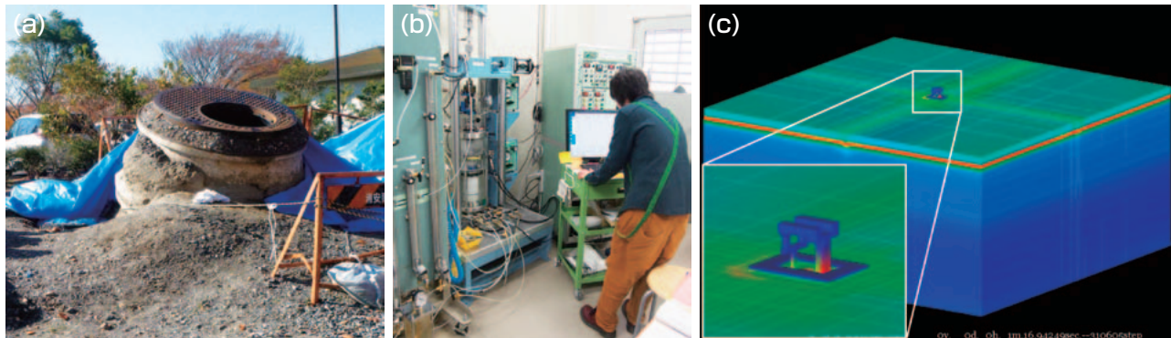
(a) 液状化によるマンホールの浮き上がり, (b) 液状化実験, (c) 液状化被害の予測シミュレーション (a) Manhole floating up due to liquefaction, (b) Liquefaction test, (c) Simulation of the damage due to liquefaction
